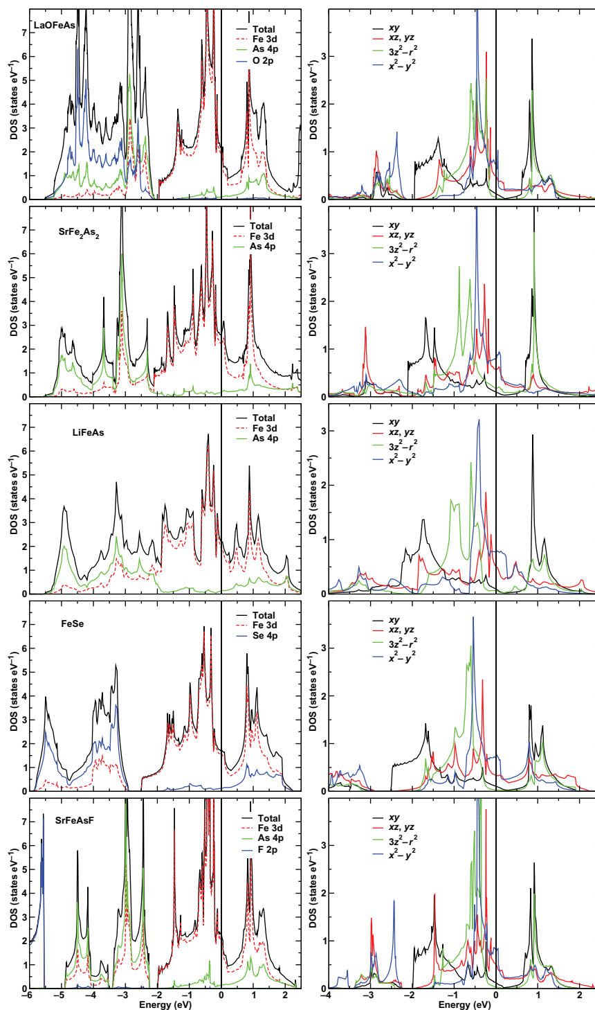
Figure 2. Comparison of total and site-resolved DOS per cell (left panel) and Fe 3d orbital-resolved DOS (right panel) of a representative member for each of the new superconducting family of compounds. LaOFeAs: 1111; SrFe 2 As 2 : 122; LiFeAs: 111; FeSe: 11; SrFeAsF: 1111'. The solid vertical lines at zero energy denote the Fermi level E_F .
