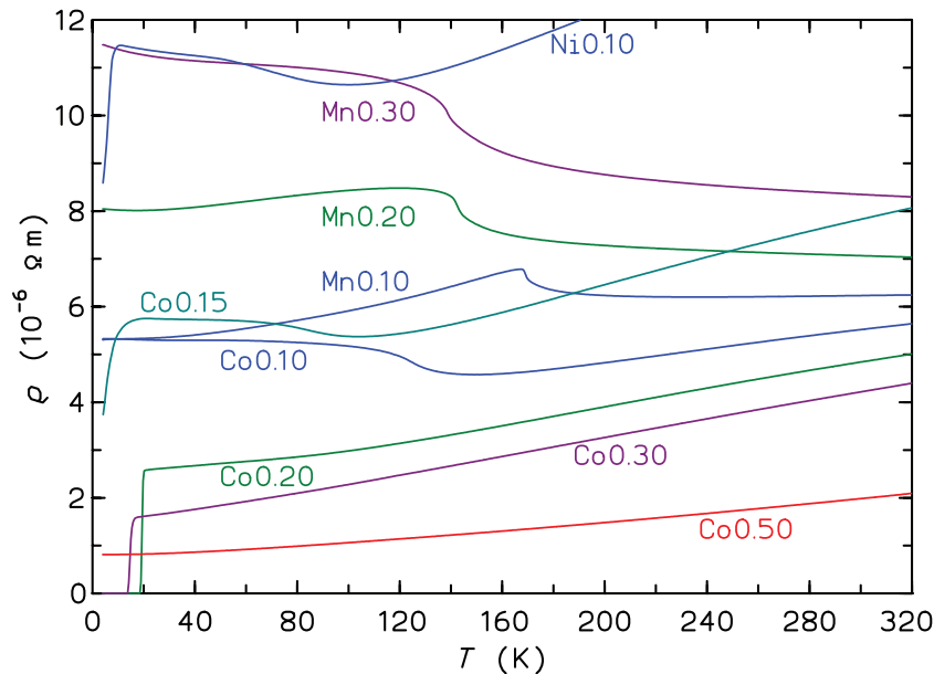
Figure 14. Electrical resistivity of polycrystalline \text{SrFe}_{2-x}\text{TM}_x\text{As}_2 ( \text{TM} = \text{Mn}, \text{Co} or \text{Ni} ) samples.
